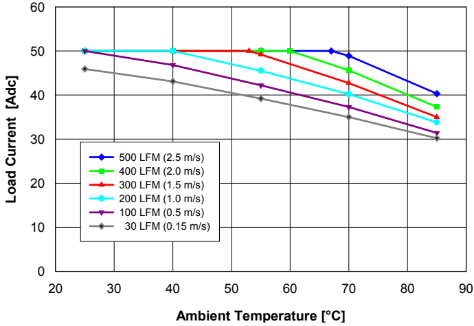
Fig. 1: Available load current vs. ambient air temperature and airflow rates for QM48T50015 converter with D height pins mounted vertically with air flowing from pin 3 to pin 1, MOSFET temperature \leq 120^{\circ}\text{C} , V_{in} = 48\text{ V} .
