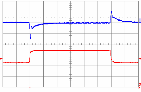
Fig. 7: Output voltage response to load current step-change (25 A – 37.5 A – 25 A) at V_{in} = 48\text{ V} . Top trace: output voltage (100 mV/div.). Bottom trace: load current (10 A/div). Current slew rate: 1 A/ \mu\text{s} . C_o = 470\text{ }\mu\text{F} tantalum + 1 \mu\text{F} ceramic. Time scale: 0.2 ms/div.
